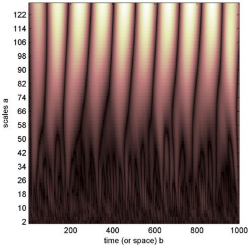
Absolute Values of C_{a,b} Coefficients for a = 2\ 4\ 6\ 8\ 10\ \dots
